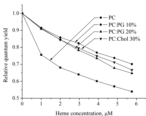
Fig. 3. Relative quantum yield of pyrene excimers. Lipid concentration was 46 \mu M.
